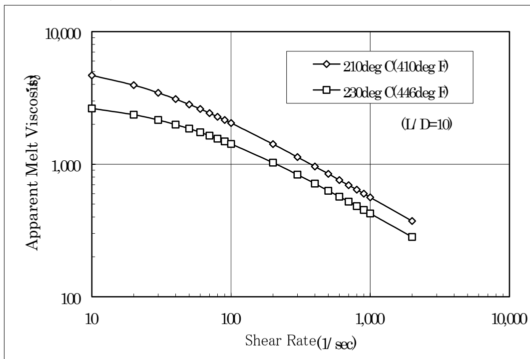
Fig.1 Melt Viscosity of Soarnol DT2903(B)
